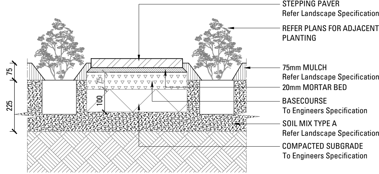
06 601 STEPPING PAVER IN GARDEN BED ON GRADE SCALE 1:10
