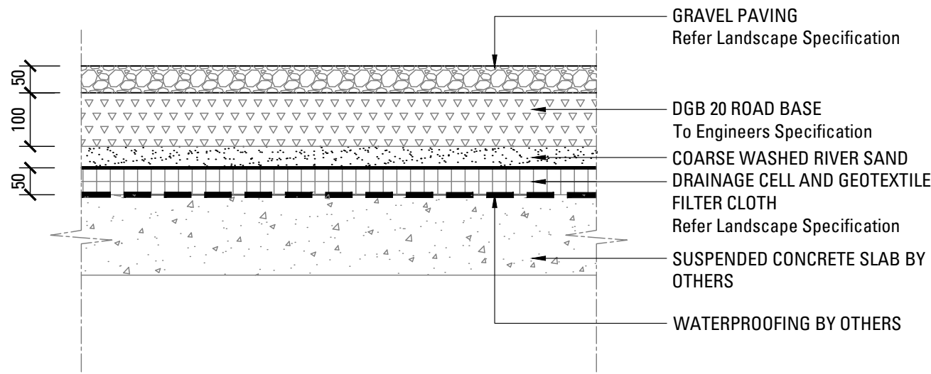
04 601 GRAVEL PAVING ON SUSPENDED SLAB SCALE 1:10
