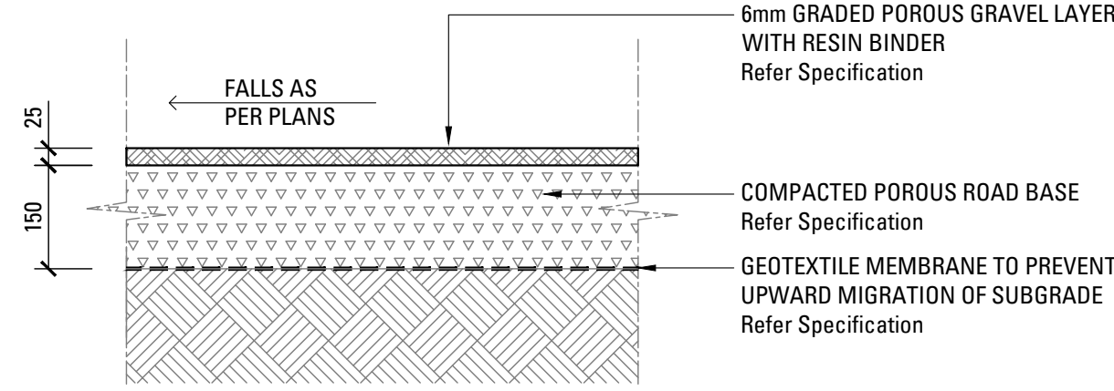
03 601 PERMEABLE GRAVEL PAVING WITH RESIN BINDER - TYPICAL DETAIL SCALE 1:10
