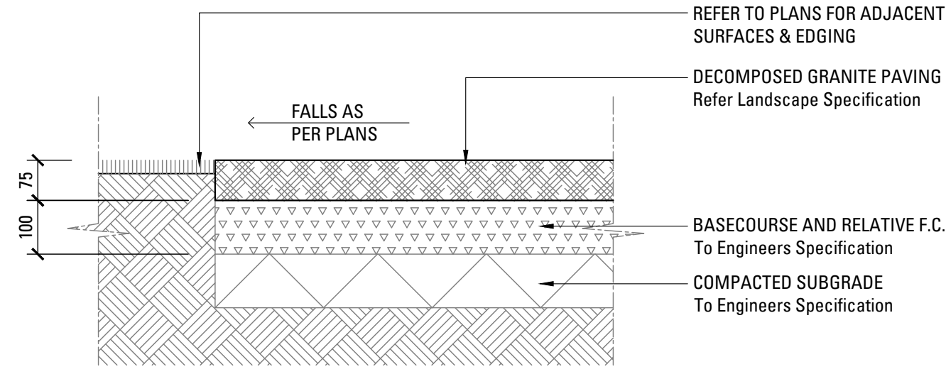
05 601 DECOMPOSED GRANITE PAVING ON GRADE SCALE 1:10
