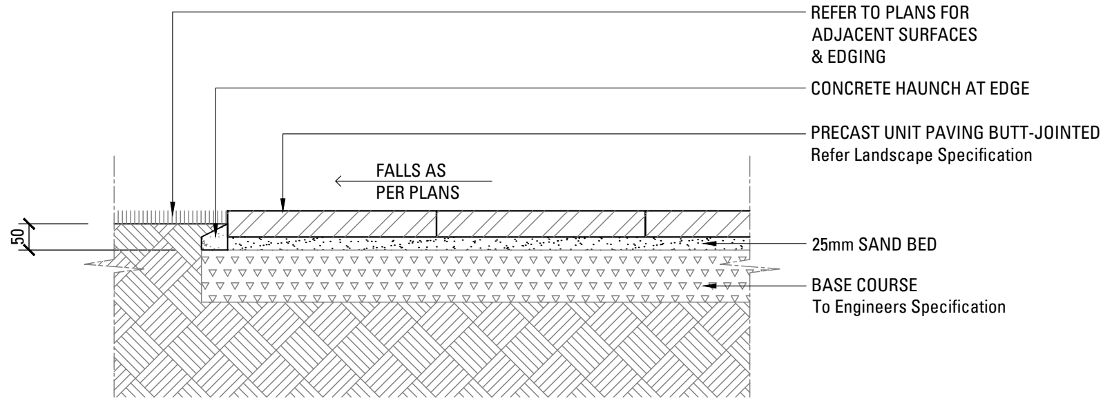
01 601 PRECAST UNIT PAVERS ON GRADE SCALE 1:10
